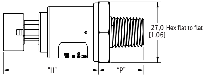
Figure 4. Pressure Port Type Mounting Dimensions (For reference only: mm/[in].) 1
