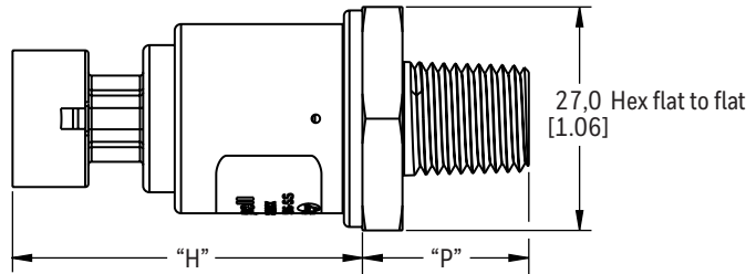
Figure 3. Electrical Connector Type Mounting Dimensions (For reference only. mm/[in].)
