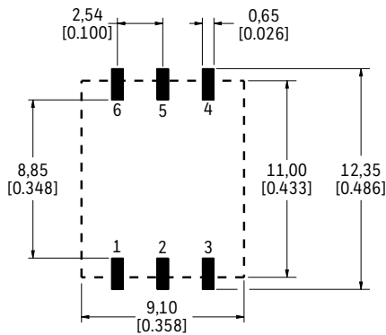
DIP Package Pressure port style DA only
