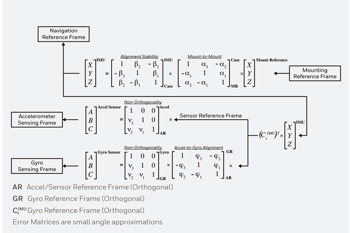
Figure 1. IMU Alignment Model
