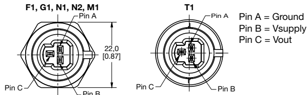
Figure 4. Metri-Pack Mounting Dimensions (For reference only, mm/[in.] )
