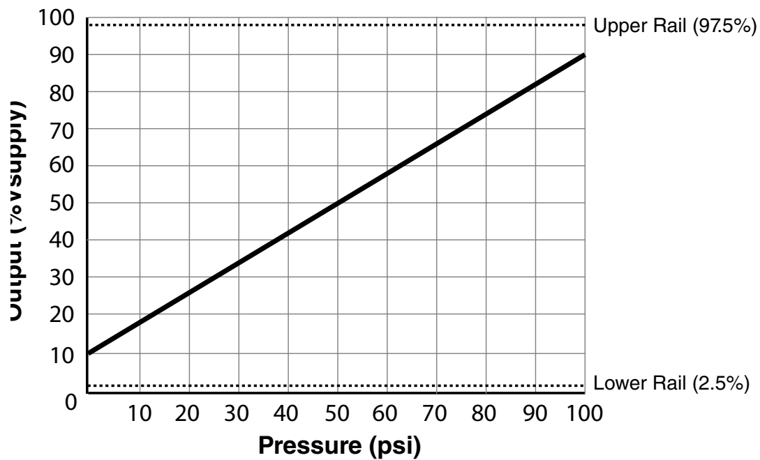
Figure 3. Analog Output with Diagnostics
