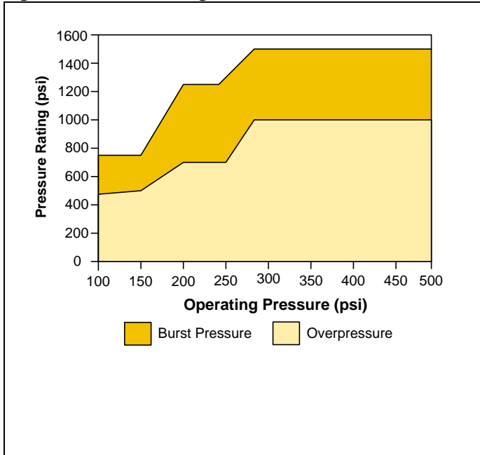
Figure 3. Pressure Rating Curve
