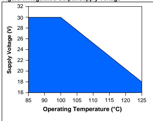
Figure 1. Regulated Output Supply Voltage
